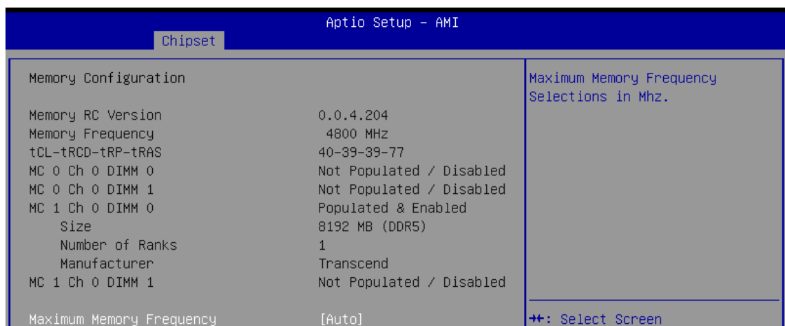
Figure 4-4-2 : Memory Information
